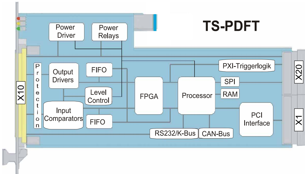
Figure 3-1 Function chart of the R&S TS-PDFT module
