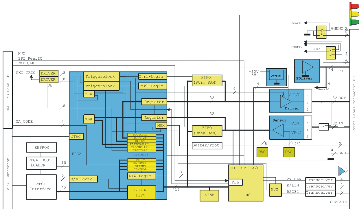
Figure 5-1 Block diagram of the R&S TS-PDFT module
