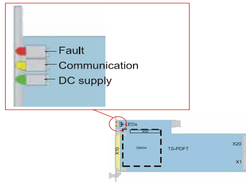
Figure 4-2 Layout of the LEDs on the R&S TS-PDFT module
