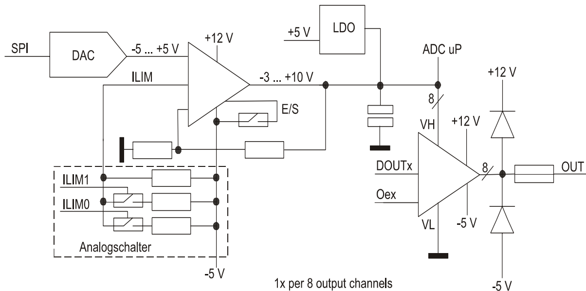
Figure 5-5 Output channel (OUTx)
