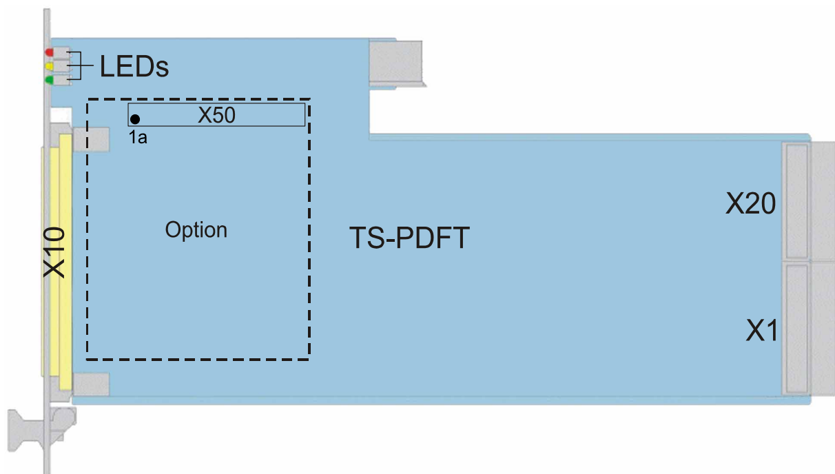
Figure 4-1 Layout of the connectors on the R&S TS-PDFT module
