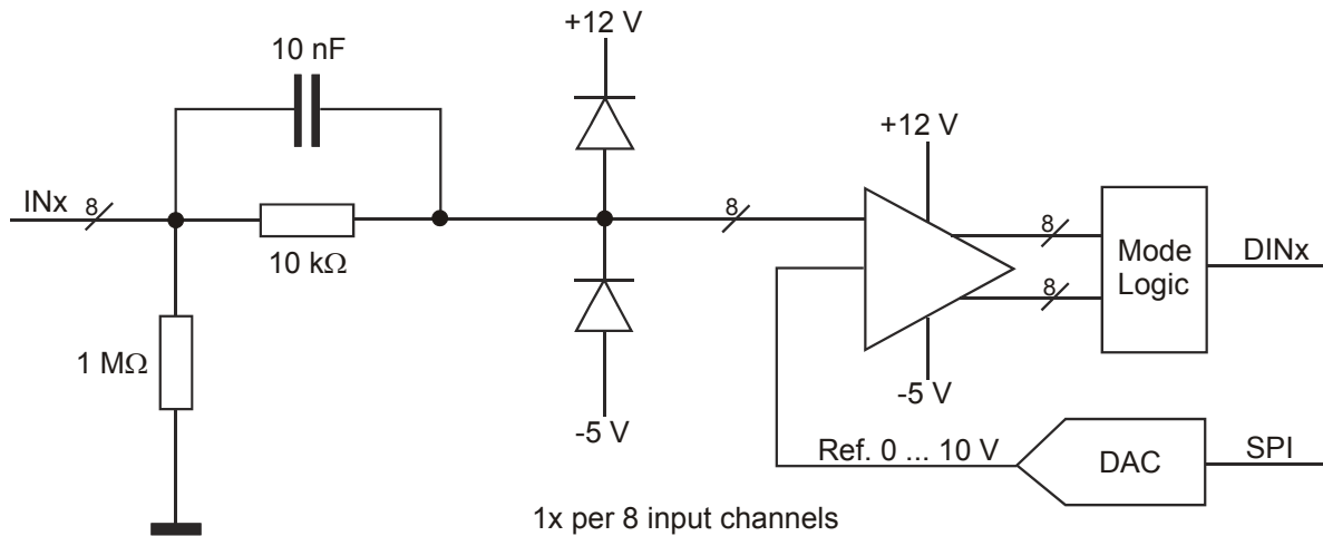
Figure 5-6 Input channel (INx)
